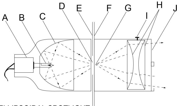
ELLIPSOIDAL SPOTLIGHT
